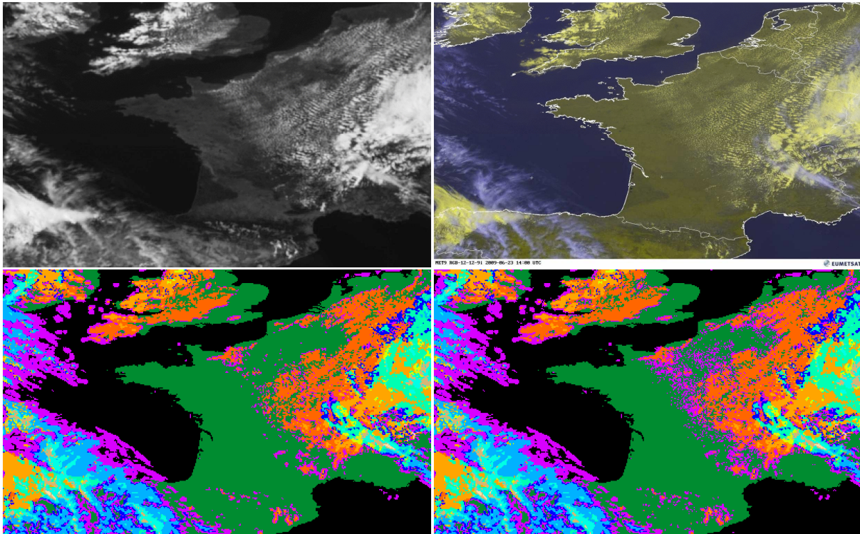
Figure 24 Fair-weather cumulus in subsident air over western Europe, 23 June 2009, 14h00UTC, (1270x770 at SEVIRI low resolution scale). Top left: enhanced 0.6 \mu\text{m} visible reflectance; top right: EUMETSAT RGB (12-12-9); bottom left: v2009 cloud type; bottom right: v2010 cloud type
