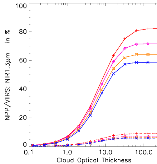
Figure 10: NPP/VIIRS simulations; solid lines: ice cloud at 200hPa, particle radius 10µm (blue), 30µm (orange), 50µm (purple), 70µm (red); dashed lines: water cloud at 600hPa, particle radius 6µm (blue), 12µm (orange), 18µm (purple), 24µm (red)
