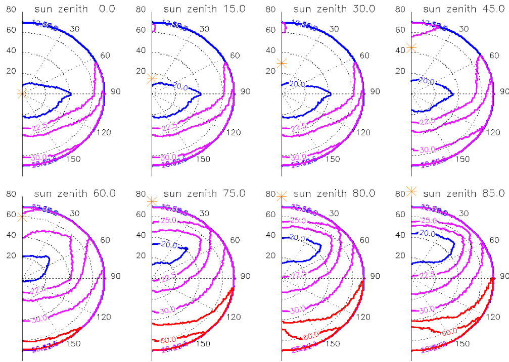
Figure 11: Polar representation of R_{1.6} threshold over snow for eight sun zenith angles.
