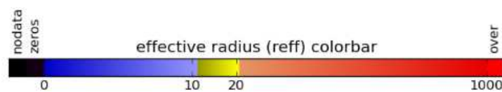
Figure 46 Example of SEVIRI cloud effective radius illustrated with the colour palette included in the CMIC NetCDF files.
